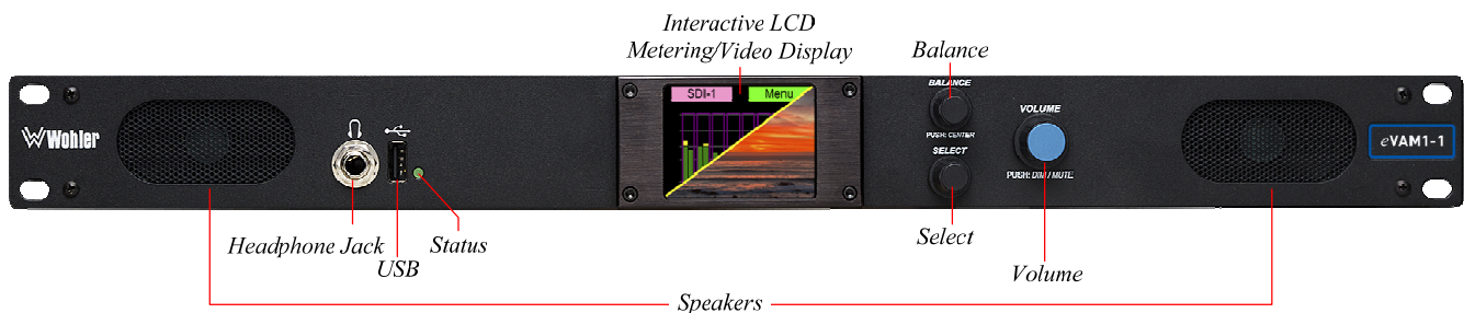
Figure 2-1: eVAM1-1 / eVAM1-1+ Front Panel
