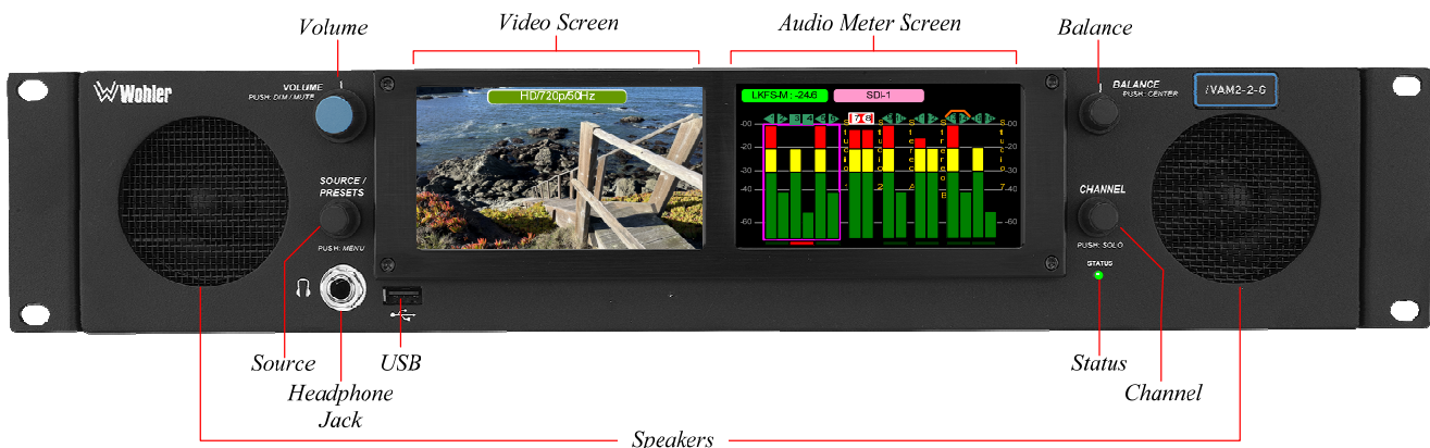
Figure 2-1: iVAM2-2-G Front Panel
