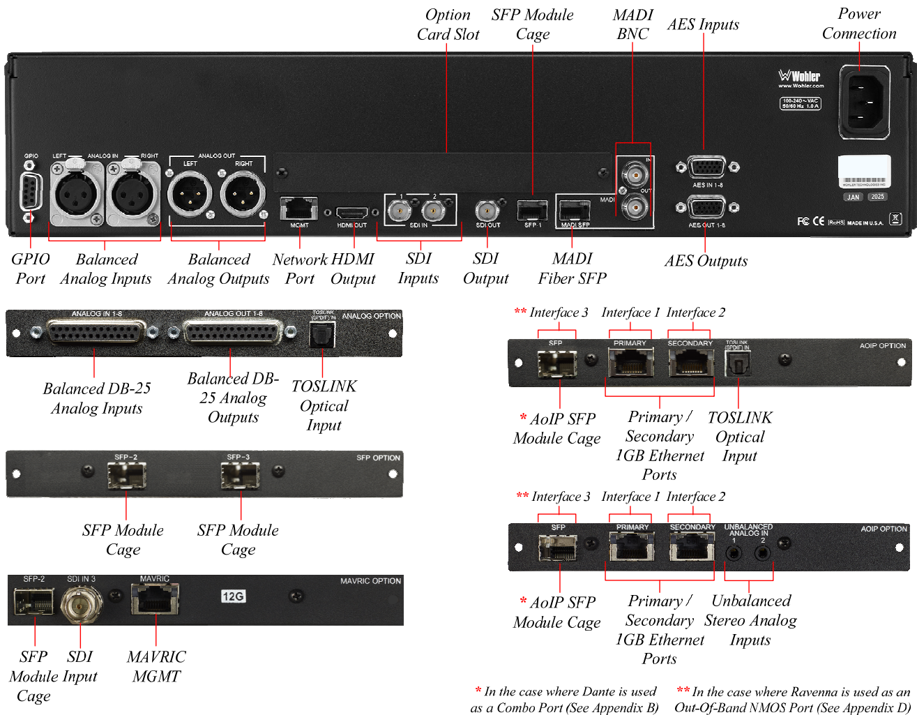
Figure 2-2: iVAM2-2-G Rear Panel & Option Cards
