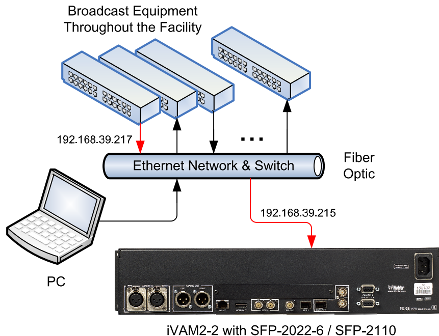
Figure 2-8: SFP-2022-6 and SFP2110 Network Diagram
