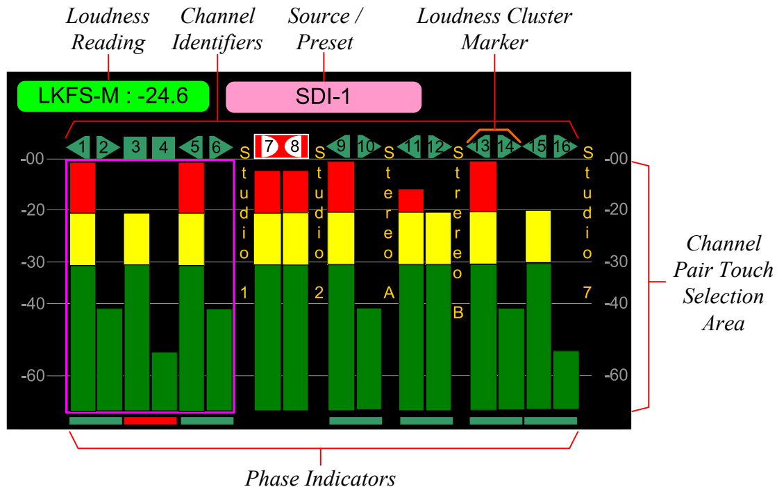
Figure 2-9: Audio Level Meter Screen
