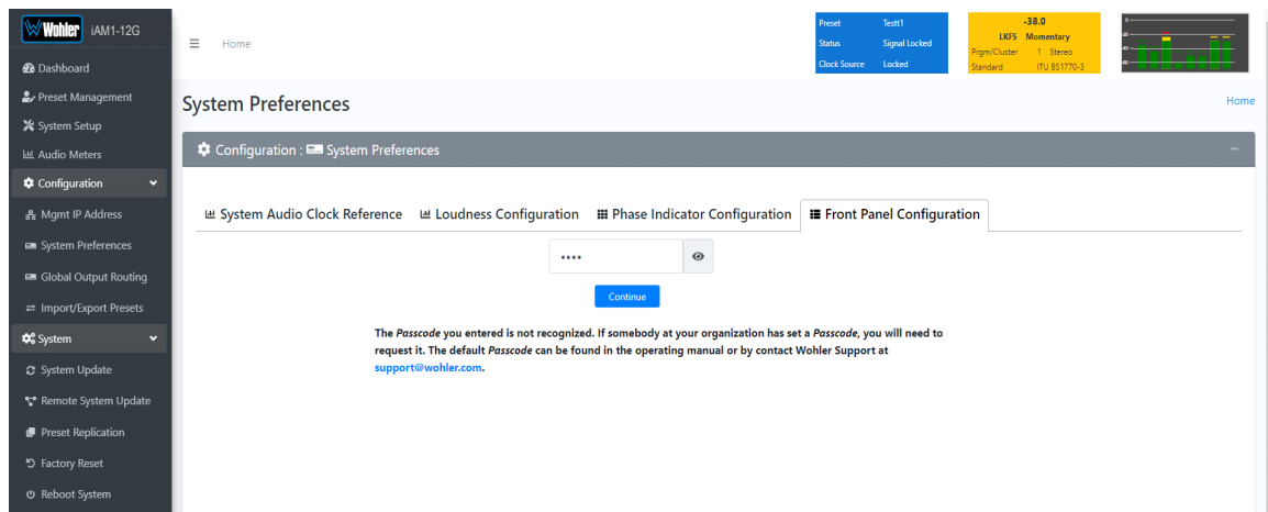
Figure 4-13: Unrecognized Passcode
