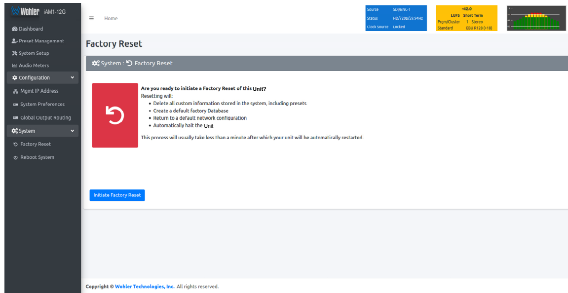
Figure 4–32: Factory Reset
