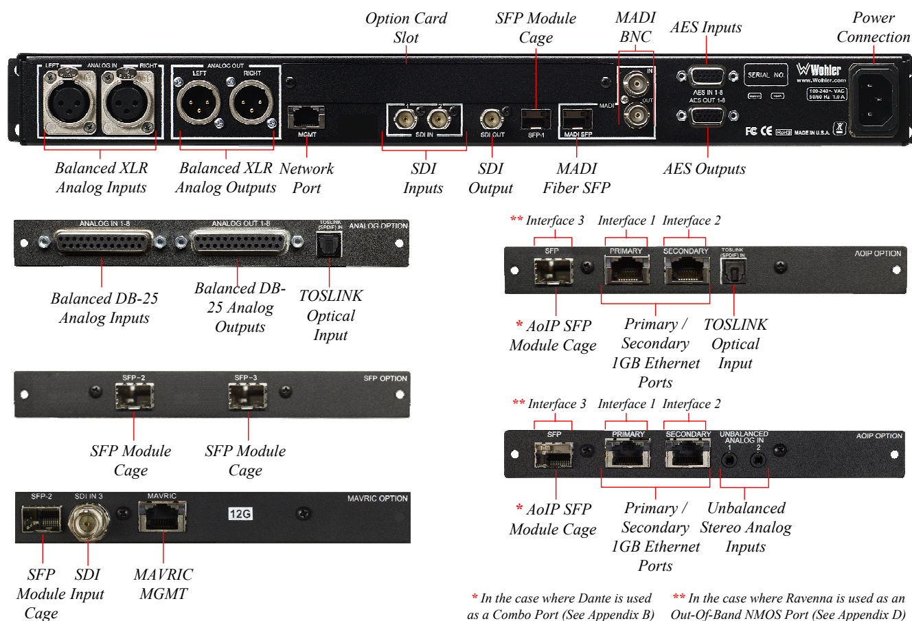
Figure 2-2: iAM1-12G Rear Panel & Option Cards
