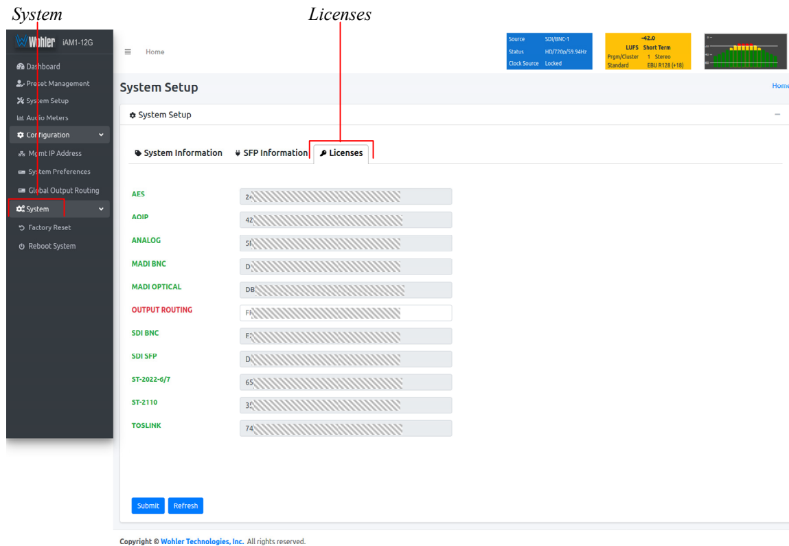
Figure 4-31: Licenses Tab
