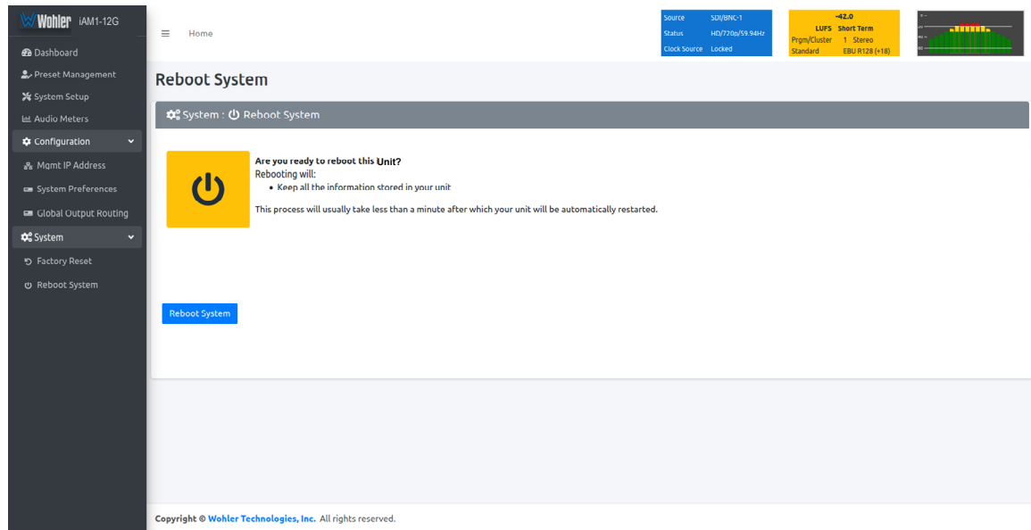
Figure 4-33: Reboot System
