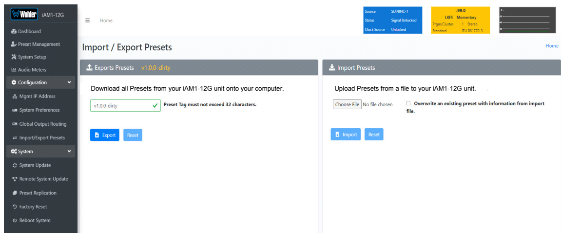
Figure 4-26: Database Export
