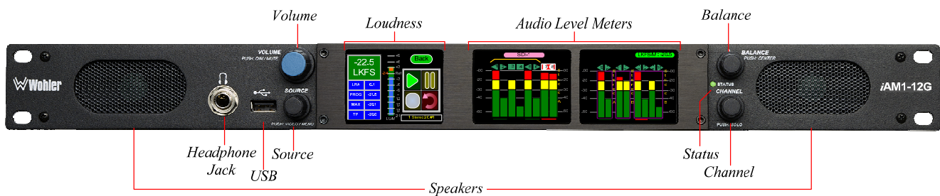
Figure 2–1: iAM1-12G Front Panel
