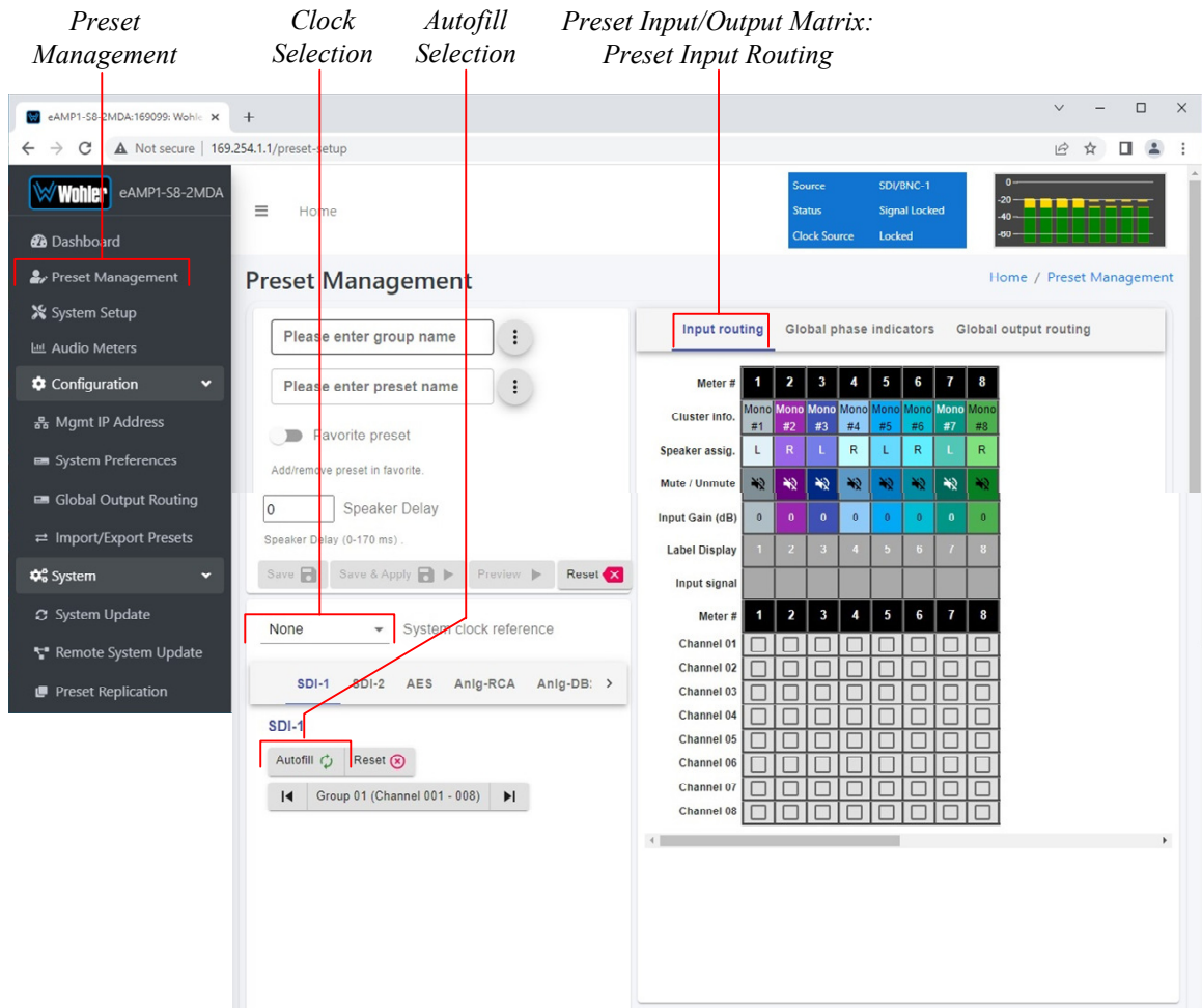
Figure 4–16: Configure Presets
