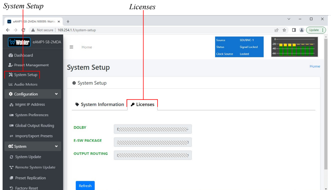
Figure 4-25: Licenses Tab
