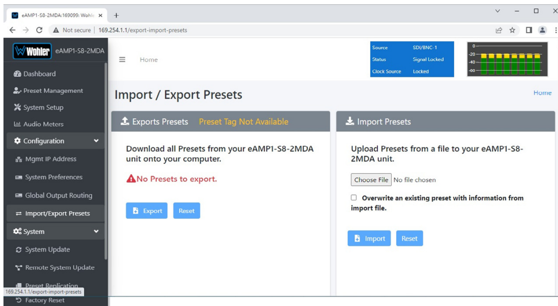
Figure 4-23: Database Export
