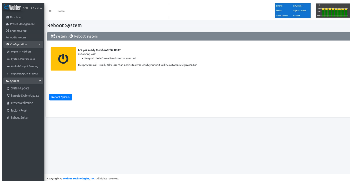
Figure 4-27: Reboot System
