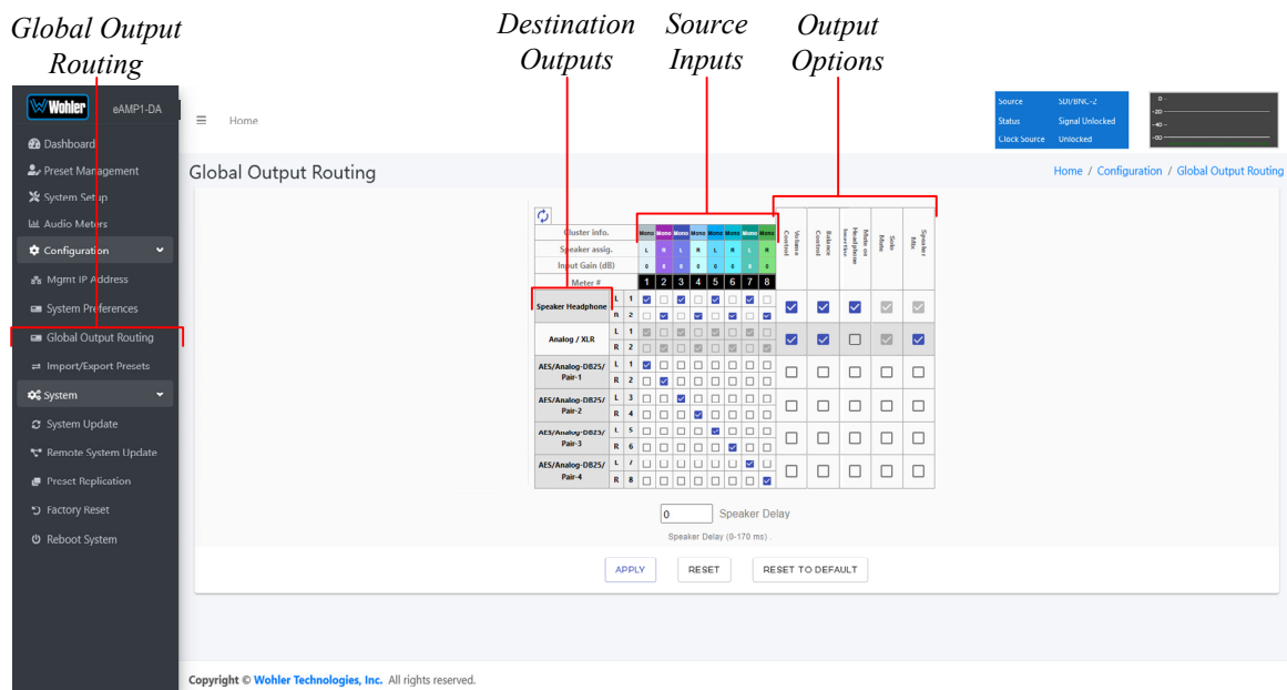
Figure 4-20: Global Output Routing
