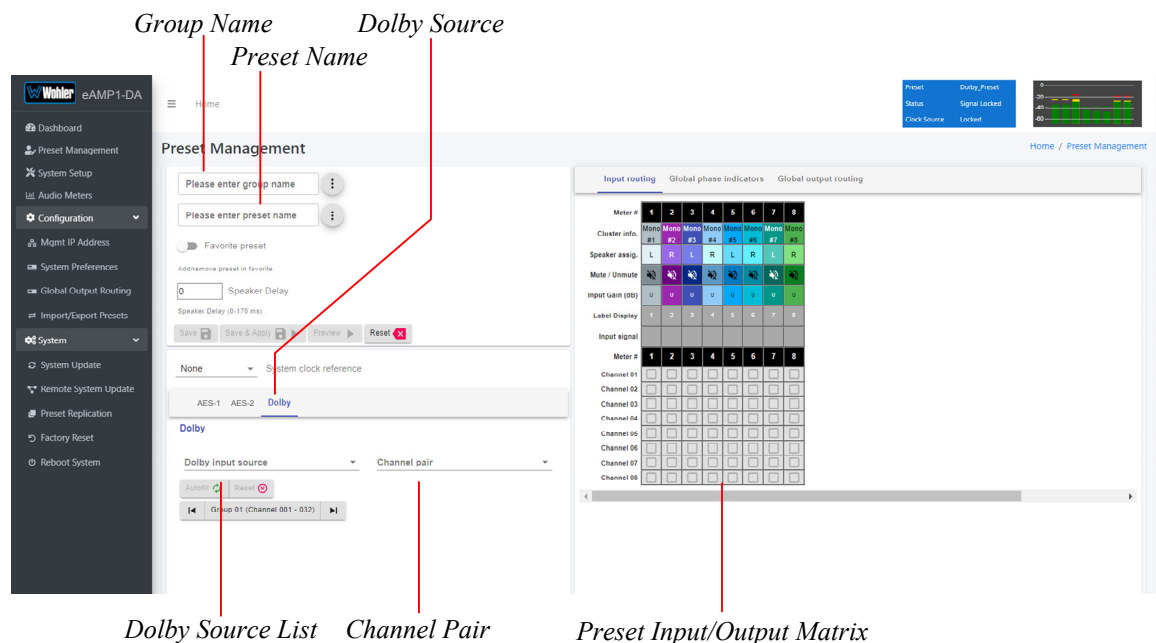
Figure 4-19: Creating a Dolby Preset
