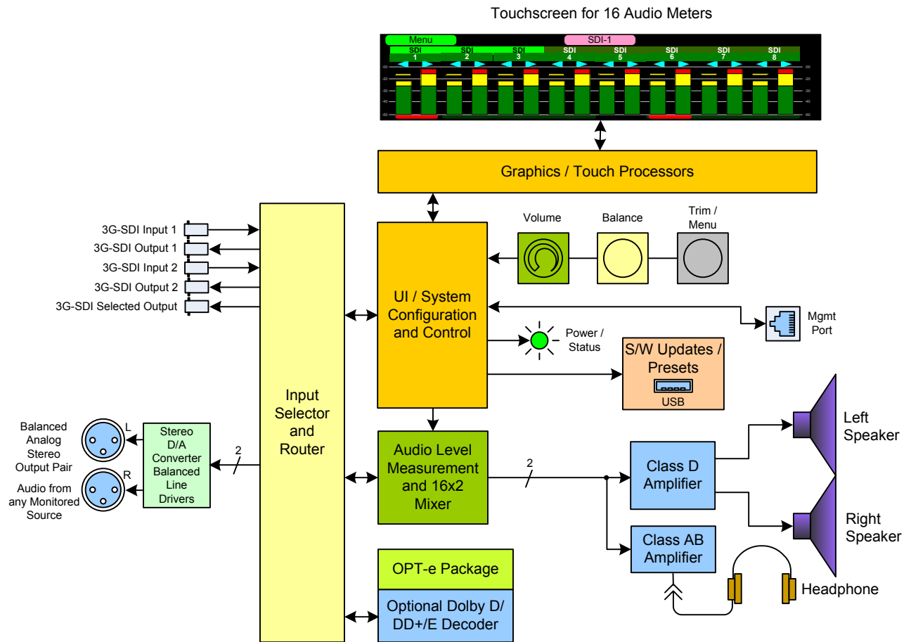
Figure 3–2: eAMP1-16M Block Diagram
