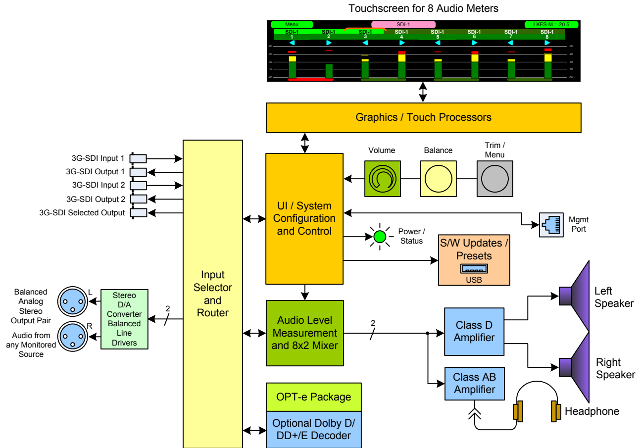
Figure 3–1: eAMP1-8M Block Diagram
