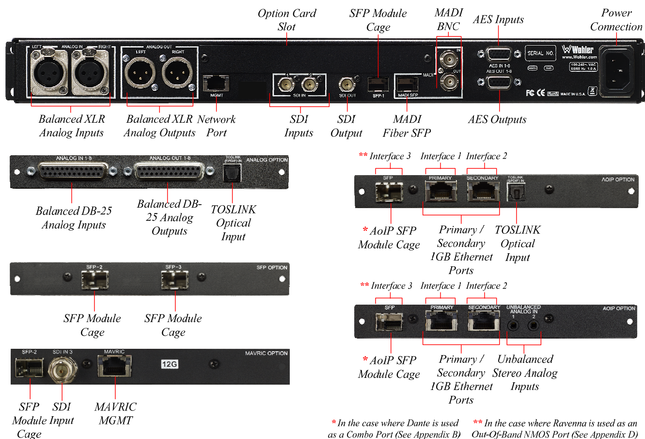
Figure 2-2: iVAM1-12G Rear Panel Layout
