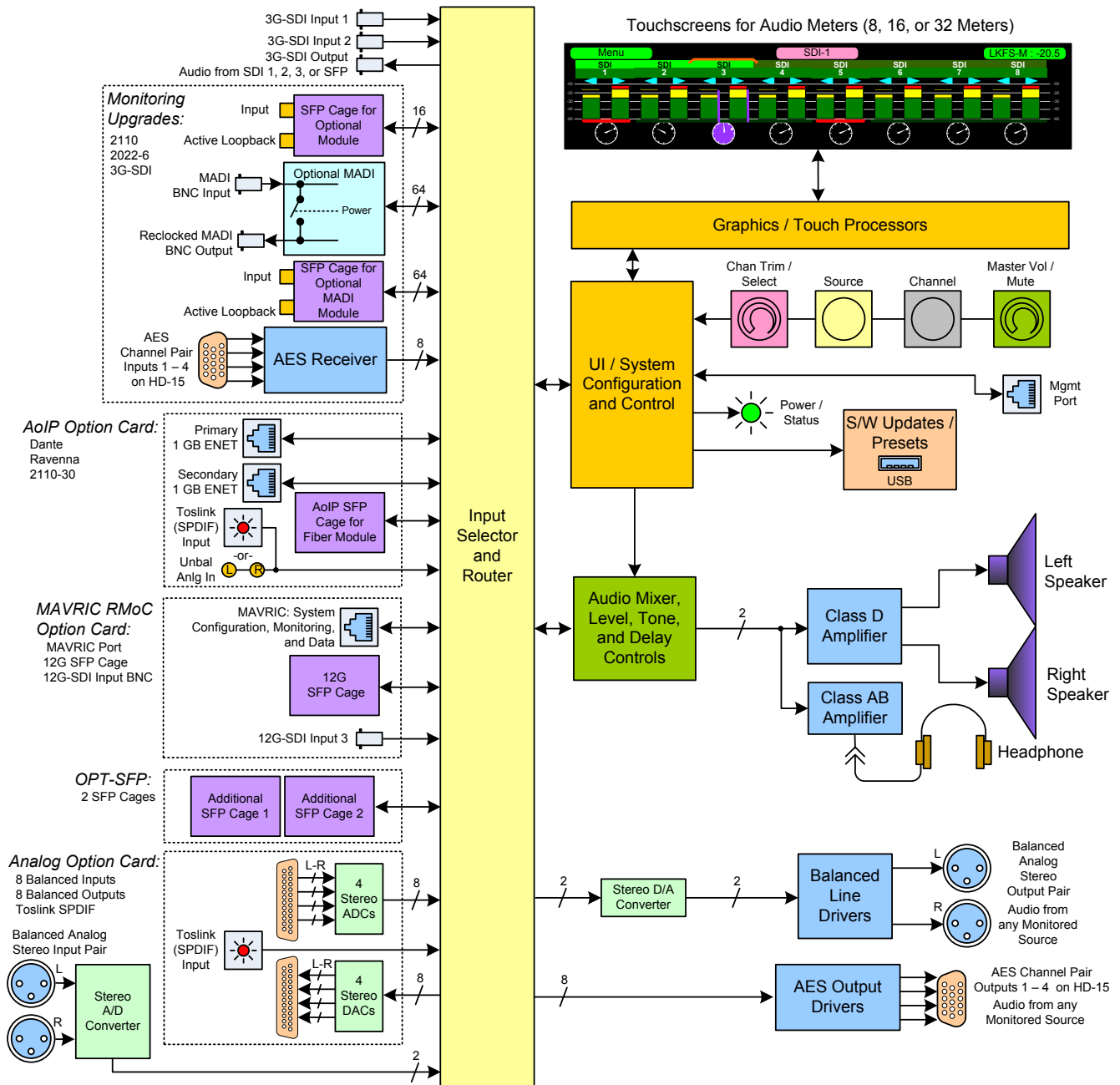
Figure 3-1: iAM-SUM Block Diagram
