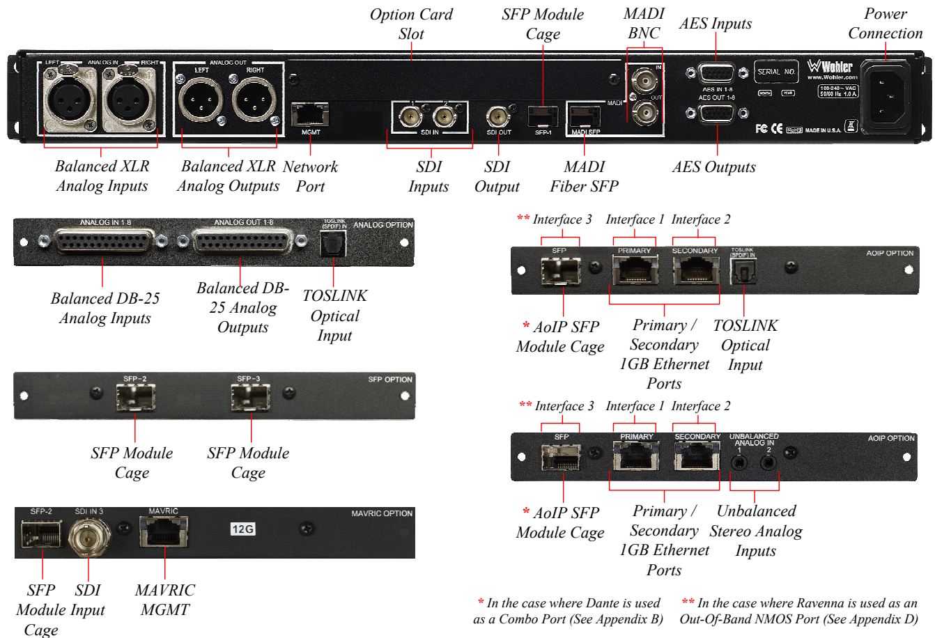
Figure 2-2: iAM-SUM Rear Panel & Option Cards
