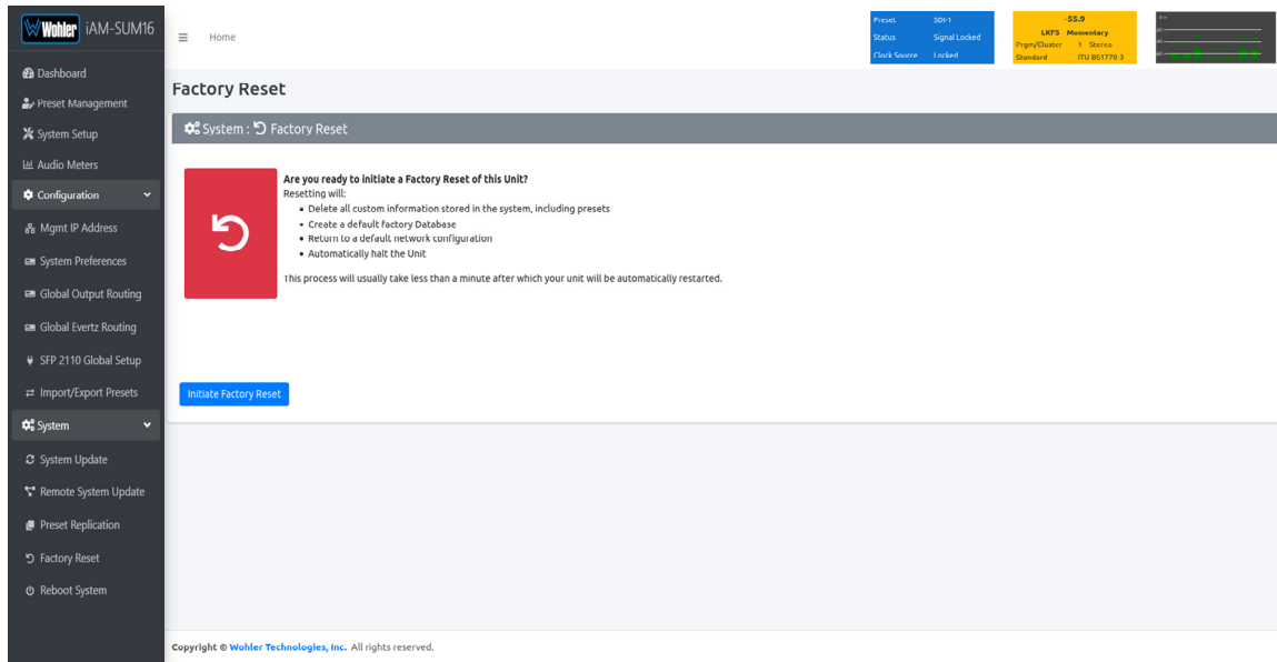
Figure 4–36: Factory Reset
