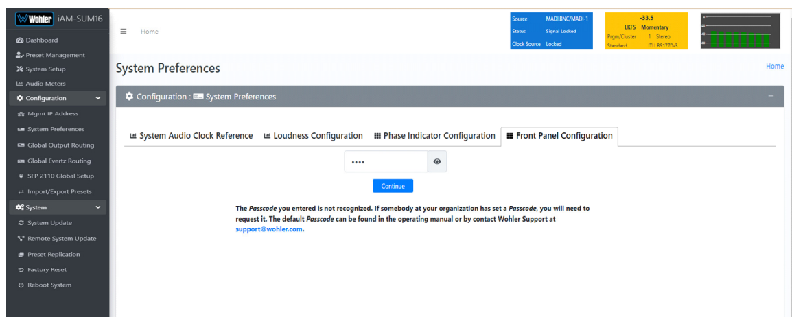
Figure 4-12: Unrecognized Passcode
