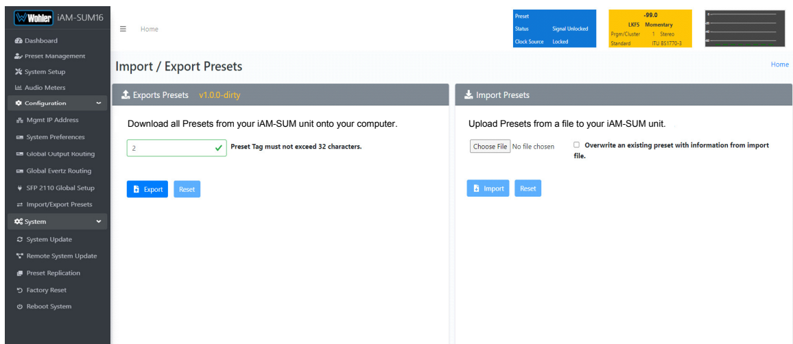
Figure 4-30: Database Export
