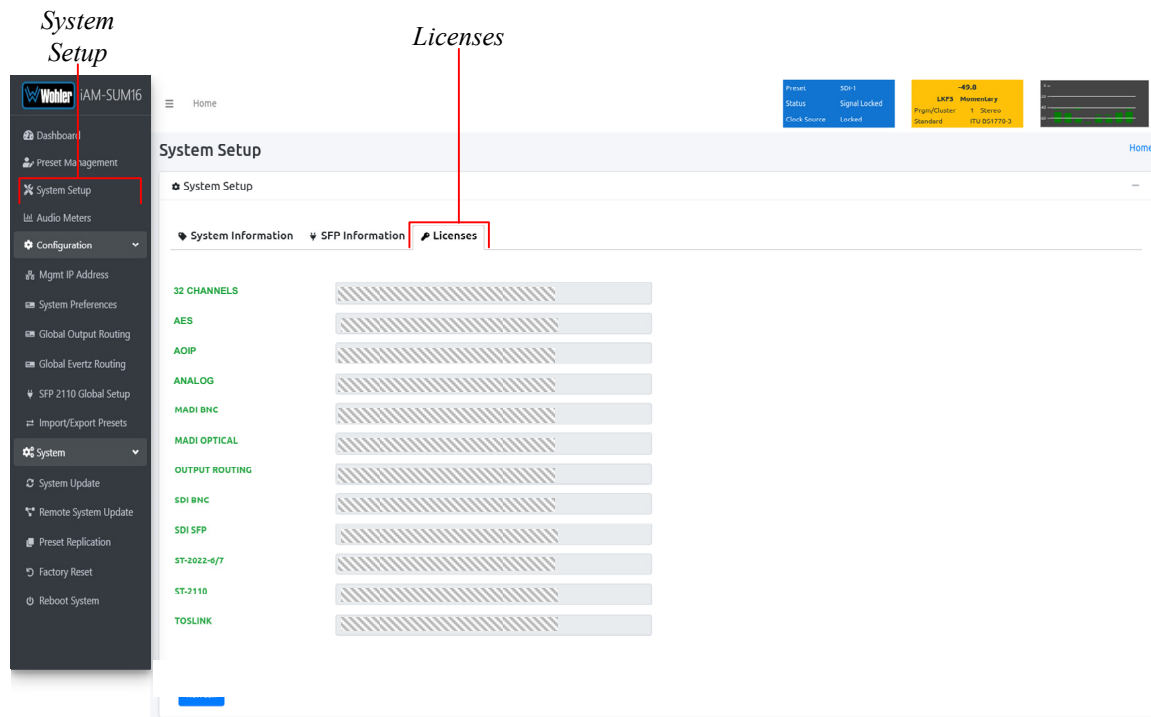
Figure 4-35: Licenses Tab
