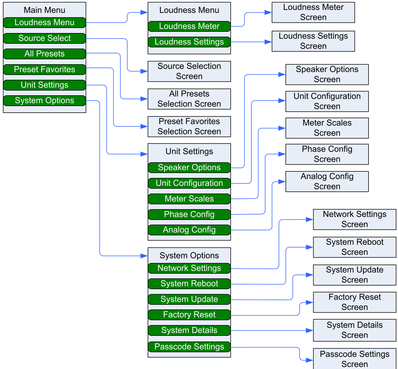
Figure 2-9: Menu Tree
