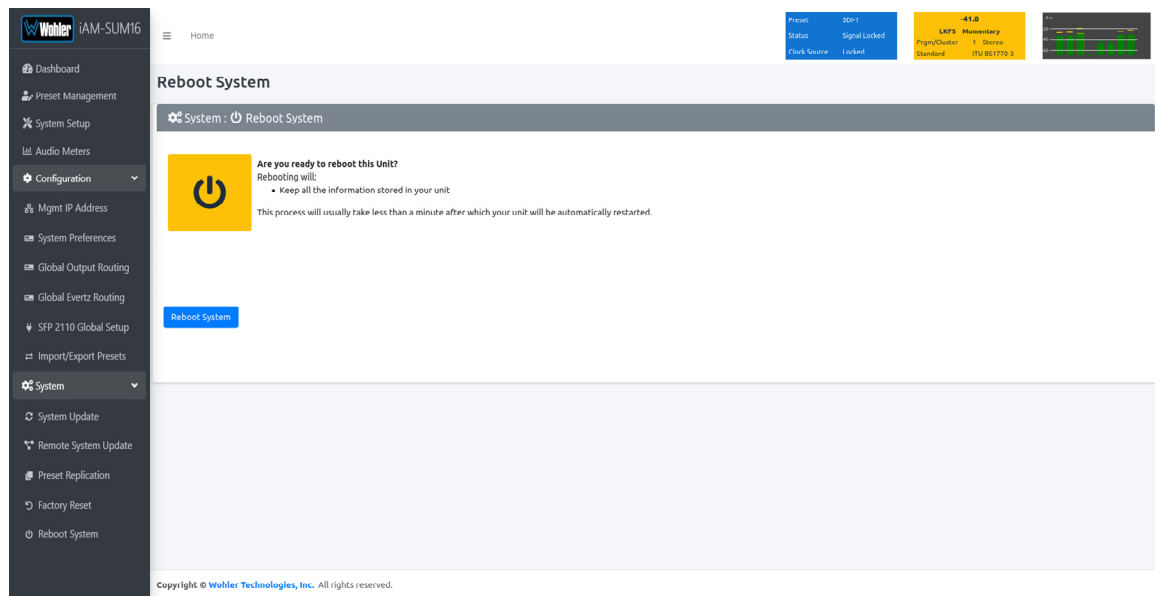
Figure 4-37: Reboot System
