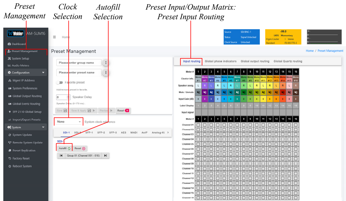
Figure 4-17: Configure Presets
