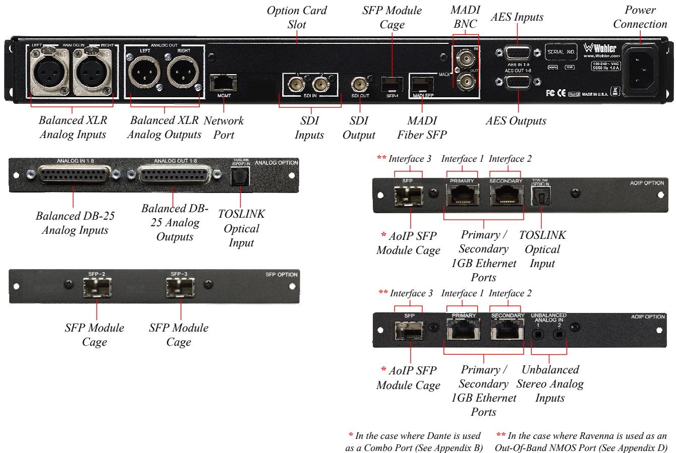
Figure 2-2: iVAM1-1 Rear Panel and Option Cards
