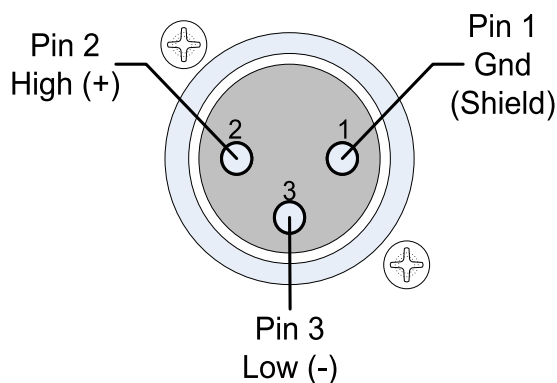
Figure 2-4: Analog XLR-F Output Connections
