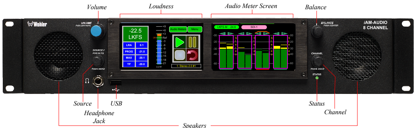
Figure 2-1: iAM2-8 Front Panel
