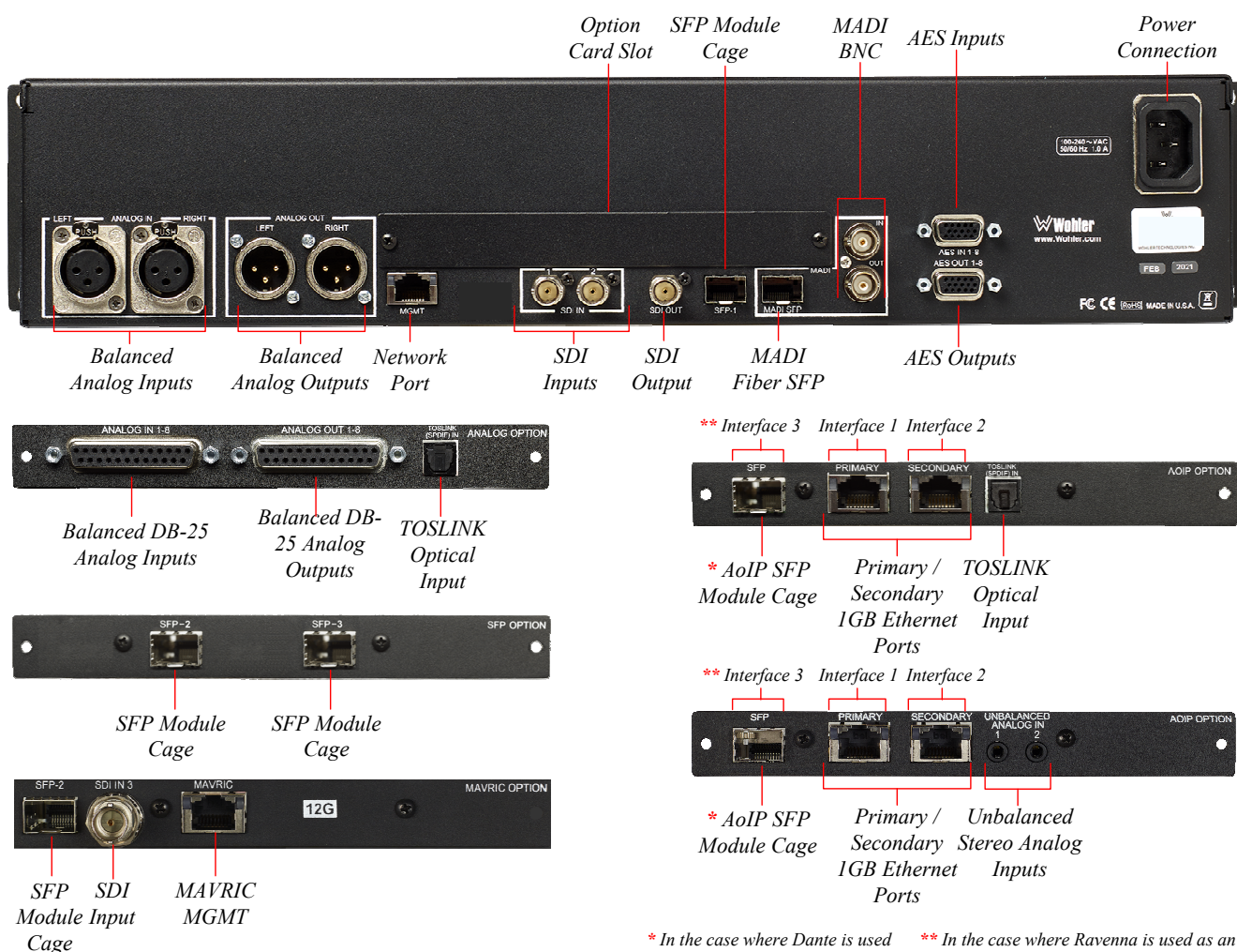
Figure 2-2: iAM2-8 Rear Panel & Option Cards
