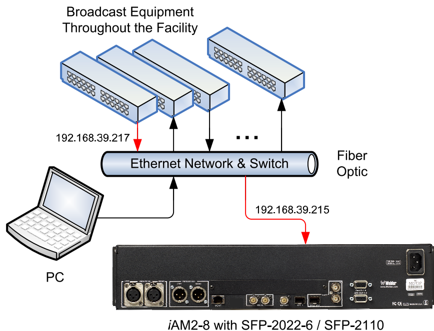
Figure 2-7: SFP-2022-6 and SFP2110 Network Diagram
