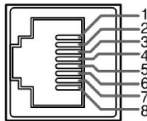
Figure 2-5: RS-485 I/O Pin-Out
