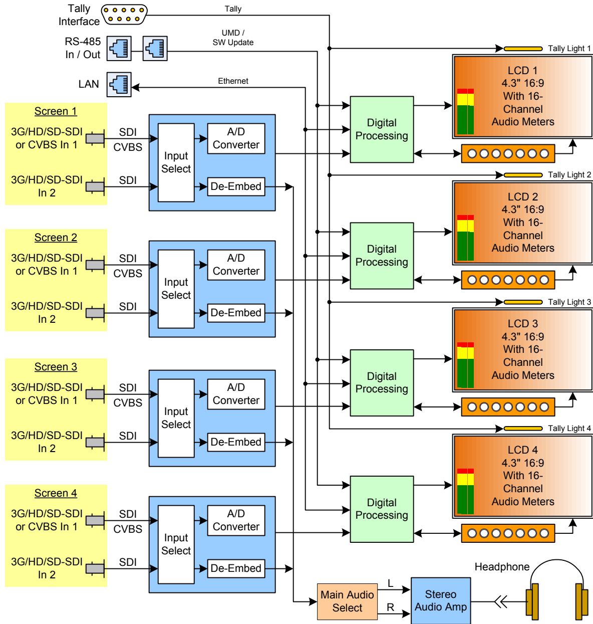
Figure 3-2: RM-2443WS-3G2 Block Diagram
